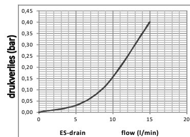
pressure loss:
